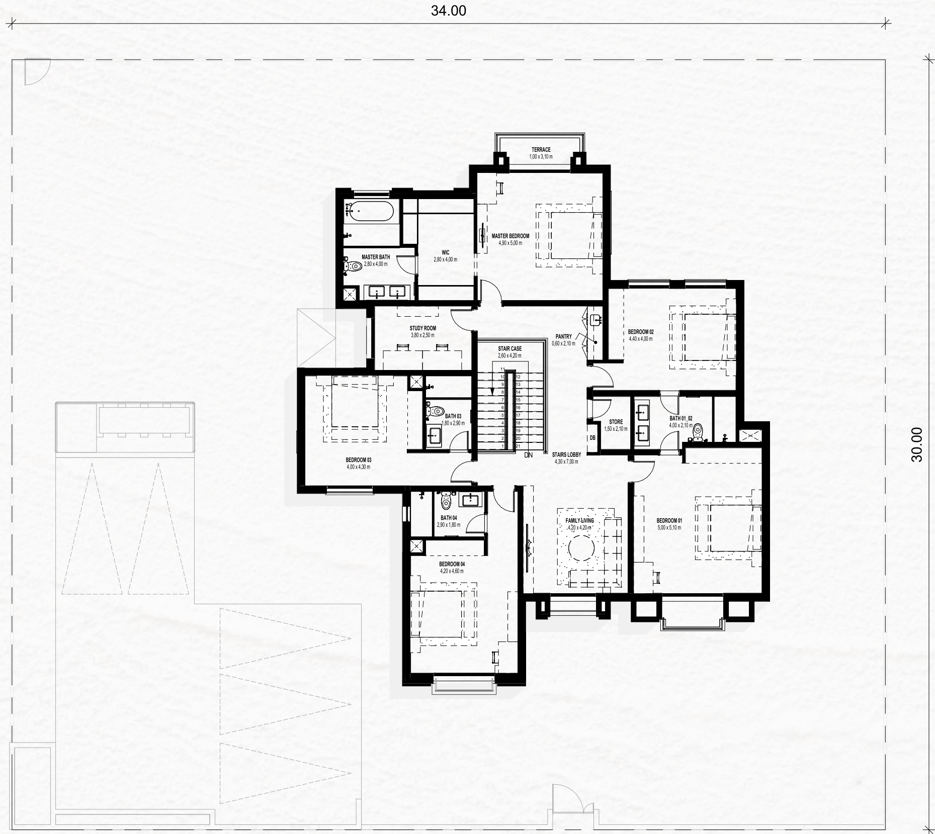
FIRST FLOOR
