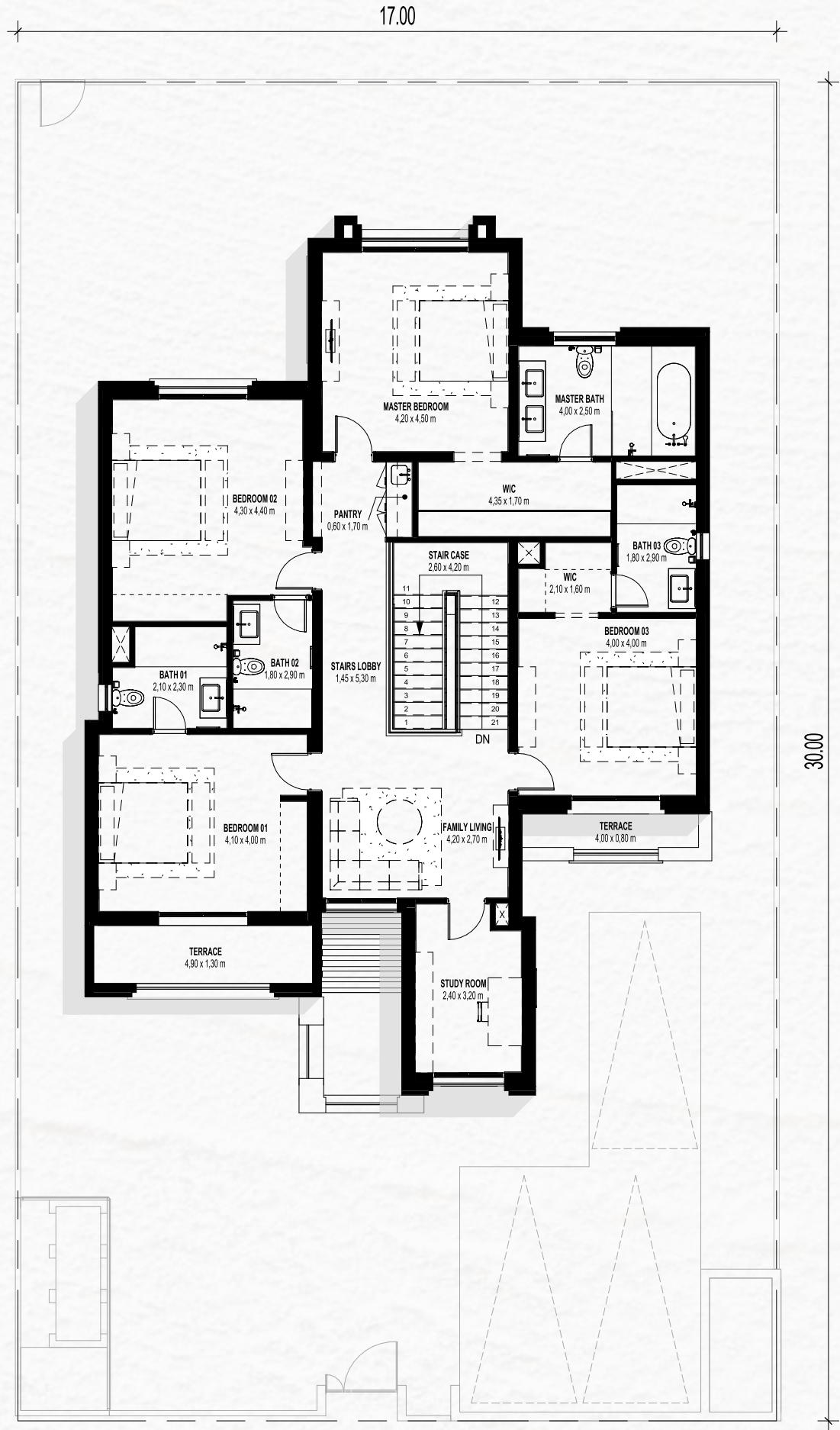
FIRST FLOOR
