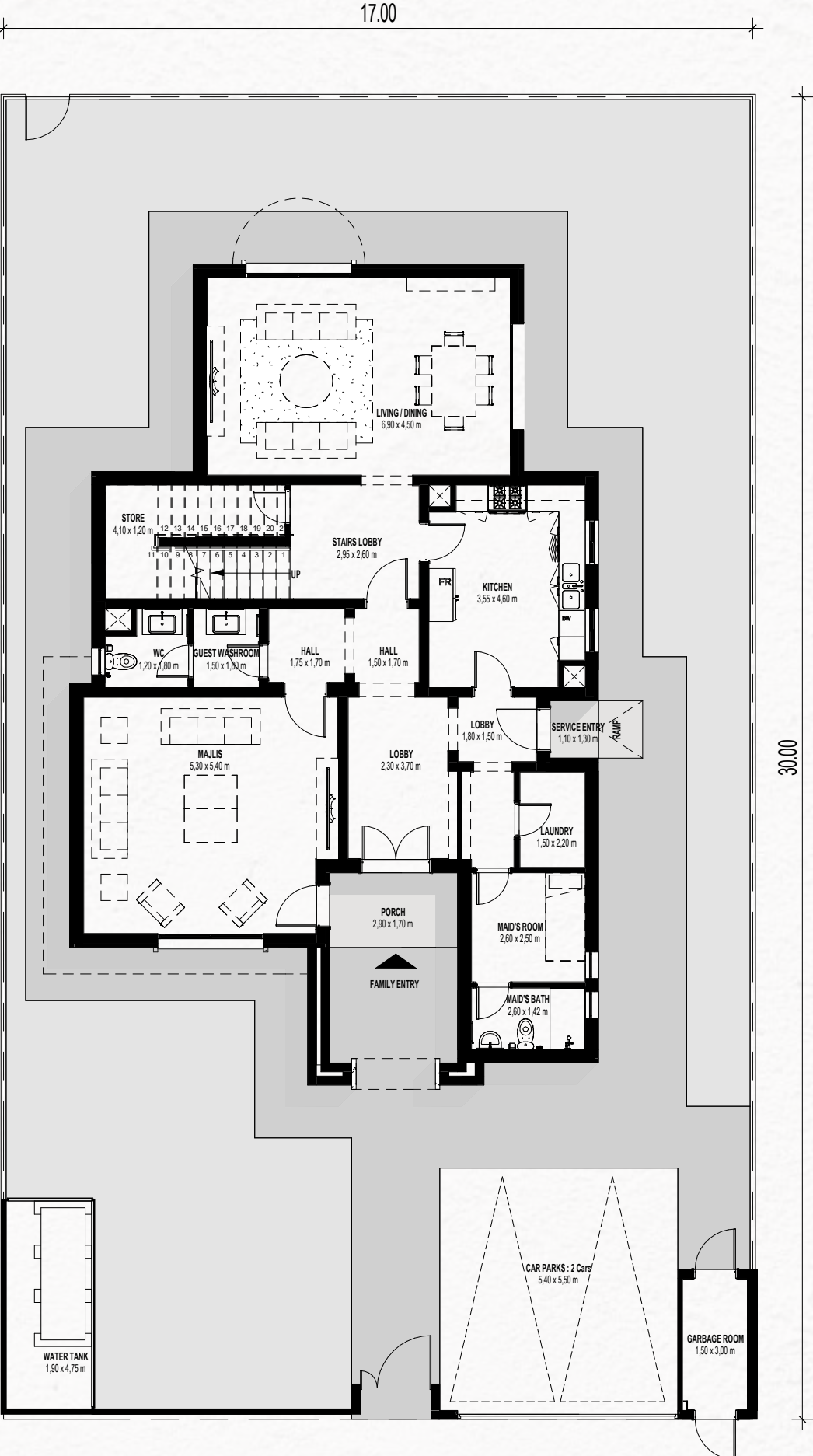
GROUND FLOOR
