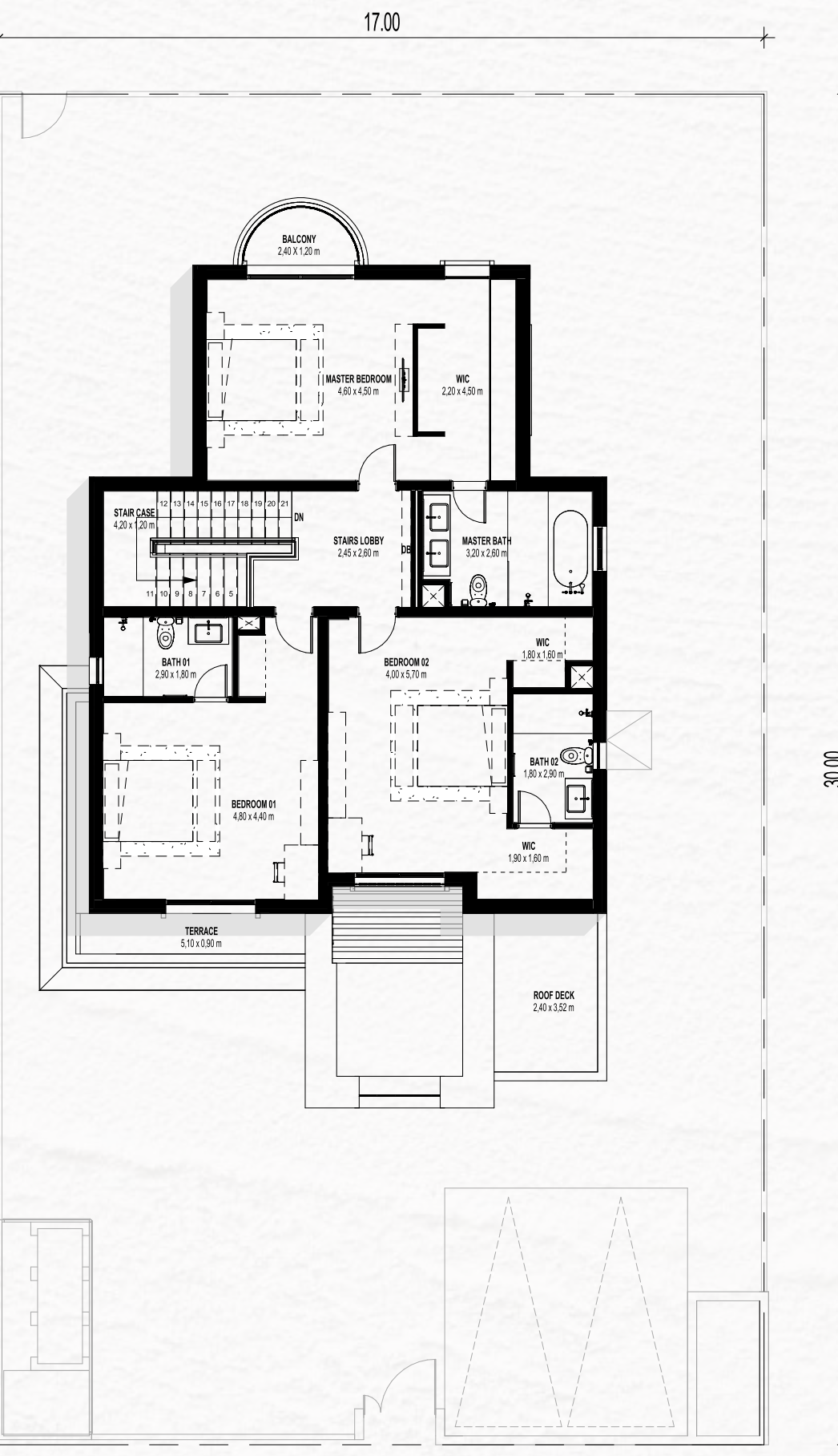
FIRST FLOOR
